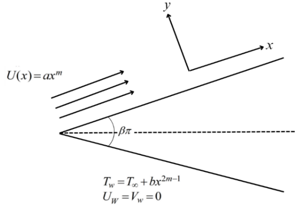
Figure 1. Falkner-Skan Flow
